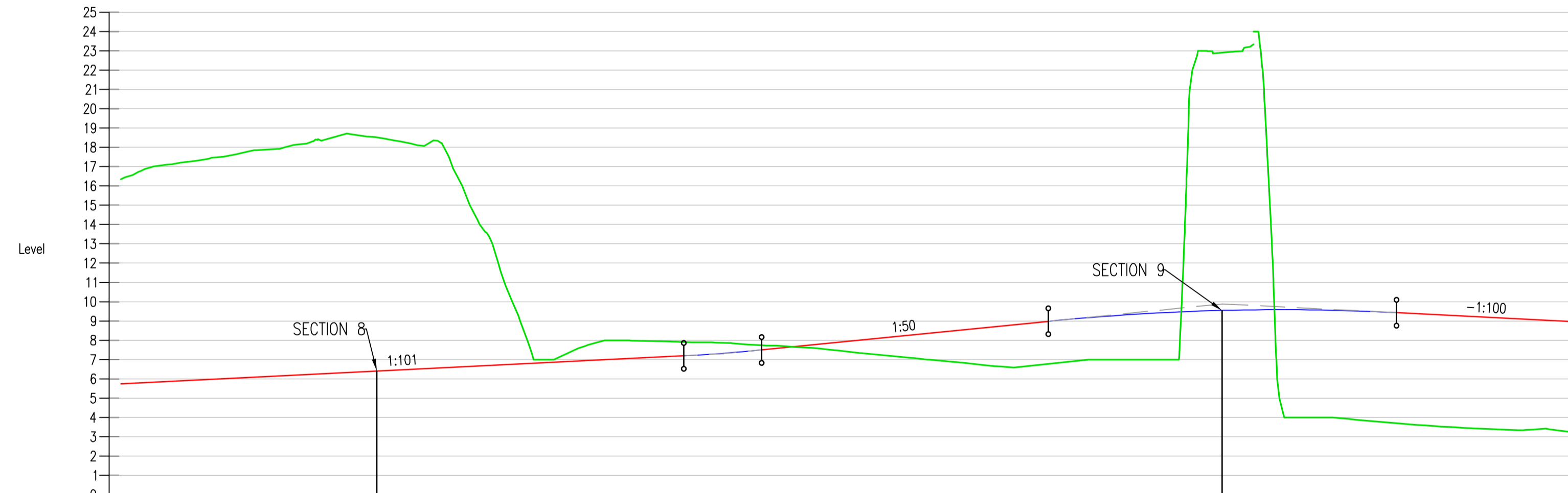
EXIT OFF RESORT ACCESS ROAD NORTH - LONGSECTION SCALE: H 1:1000, V 1:200
