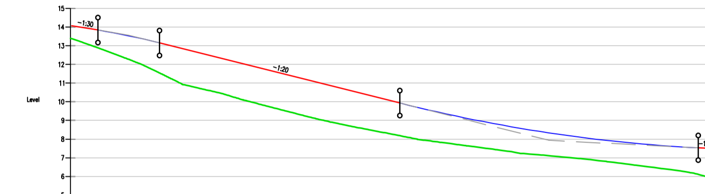
Alignment - Access Northbound SCALE: H 1:1000, V 1:200. DATUM: 5.000
