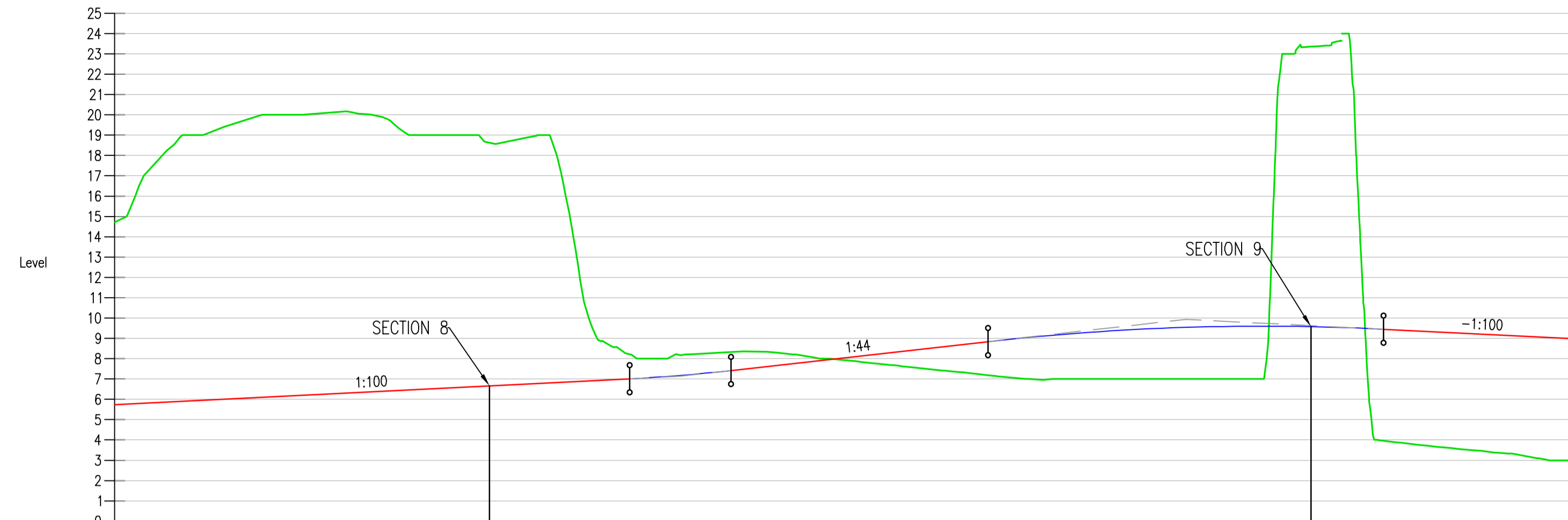
EXIT OFF RESORT ACCESS ROAD - LONGSECTION SCALE: H 1:1000, V 1:200
